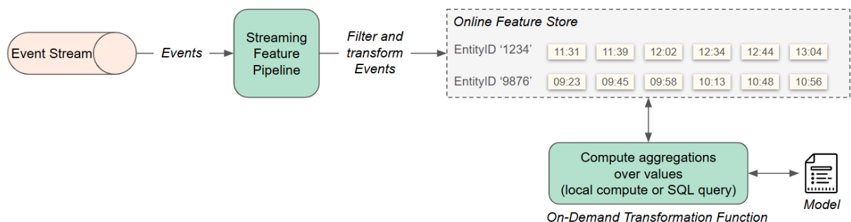
Figure 9-4. Shift right architecture that filters and transforms events in a streaming feature pipeline before they are written to the online feature store. ODTs compute aggregations from the events either locally with DataFrames or using a pushdown aggregation SQL command.
