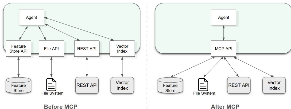
Figure 12-5. Model Context Protocol (MCP) is a protocol for standardizing how agents can perform actions and retrieve data from external tools and services.
