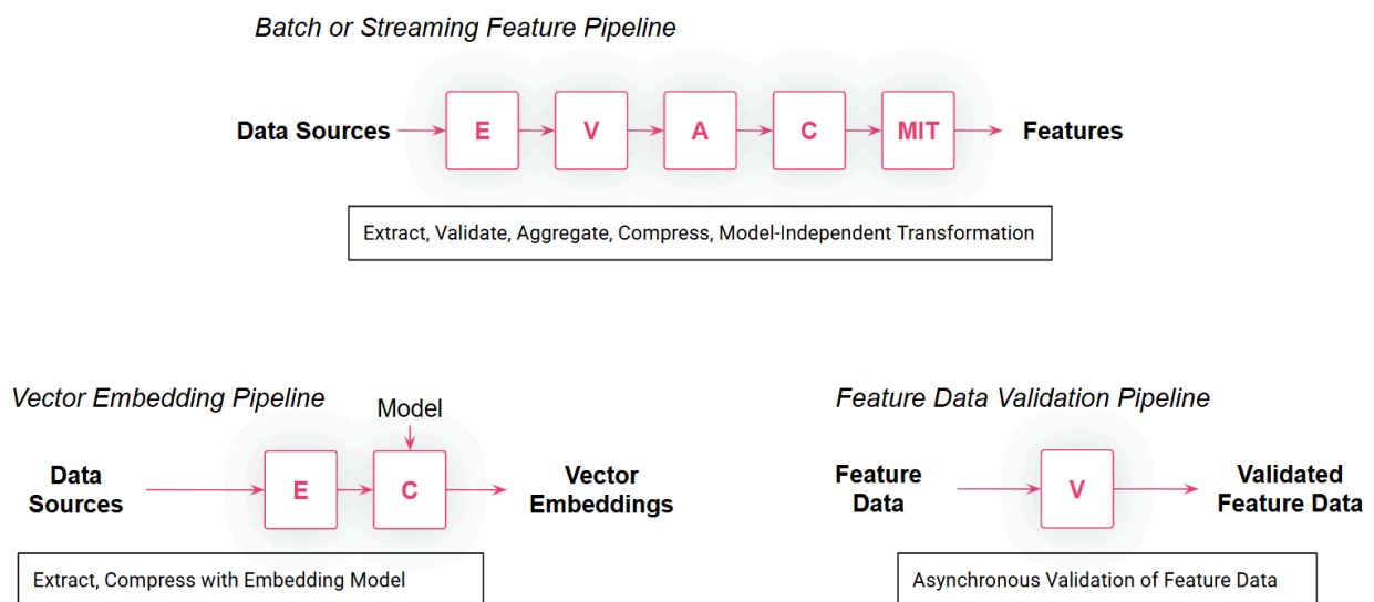
Figure 2-7. Classes of feature pipeline
