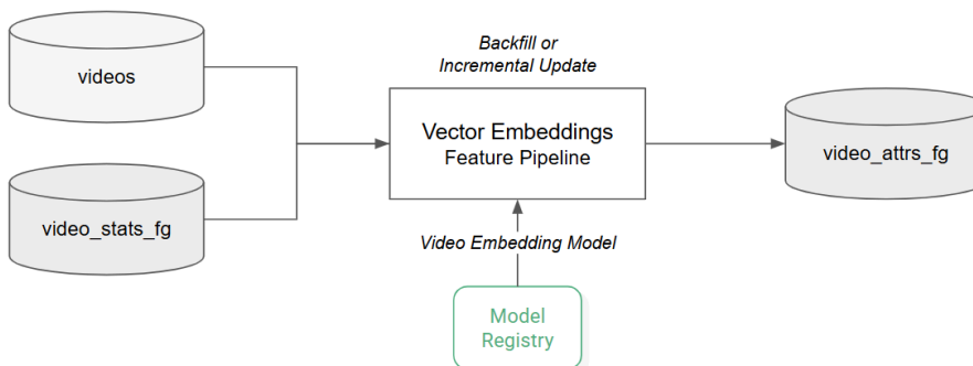
Figure 15-5. The vector embedding pipeline periodically updates the vector index with new videos and new video statistics.
