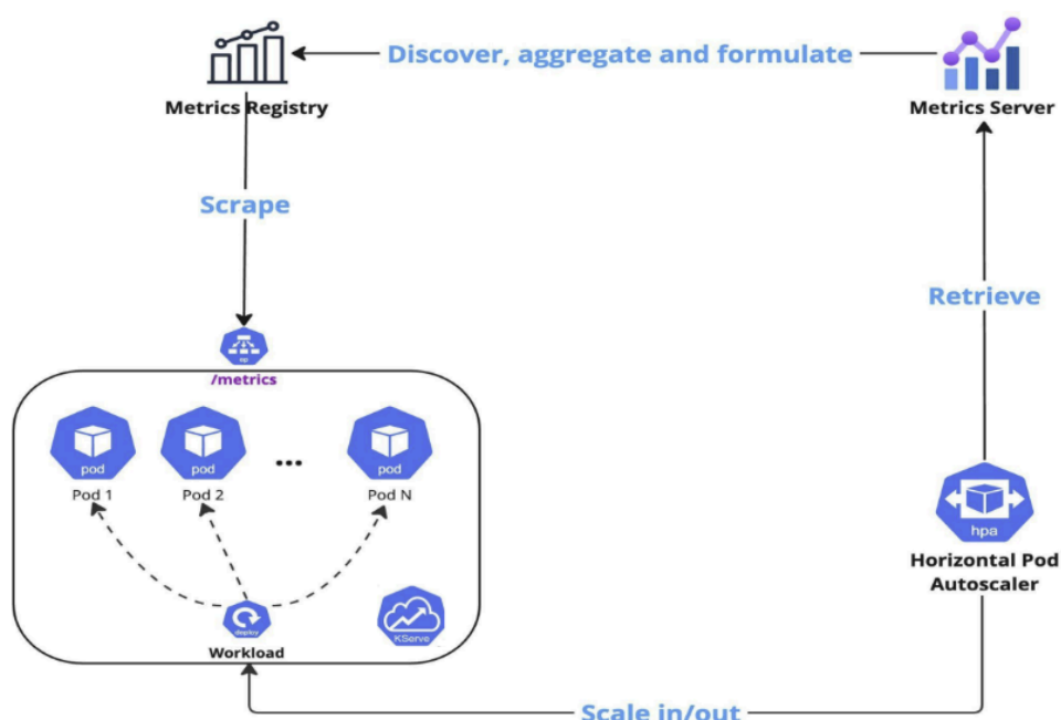
Figure 14-4. Metrics-driven auto-scaling architecture in Kubernetes. A metrics registry scrapes metrics from the target pods and aggregates them in a metrics server. A horizontal pod autoscaler uses the metrics to drive scale-in and scale-out decisions, adding or removing redundant pods as the load increases or decreases, respectively. [Image from public domain]
