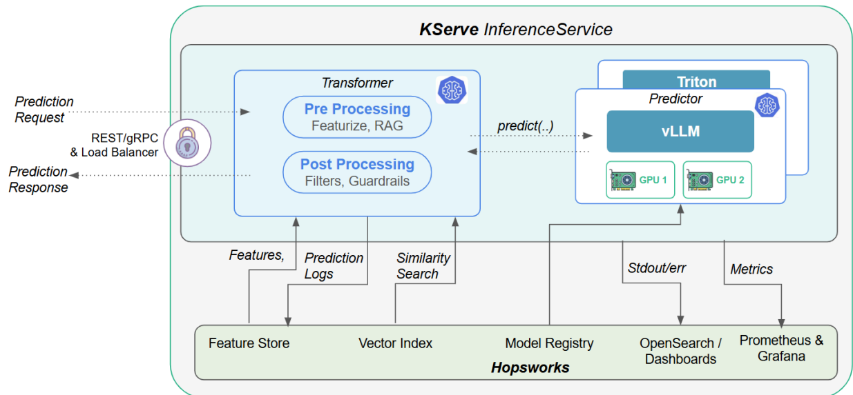
Figure 11-7. Model Deployments on KServe can use infrastructural services provided by Hopworks, including security, logging, monitoring, RAG, feature store, and GPU management.
