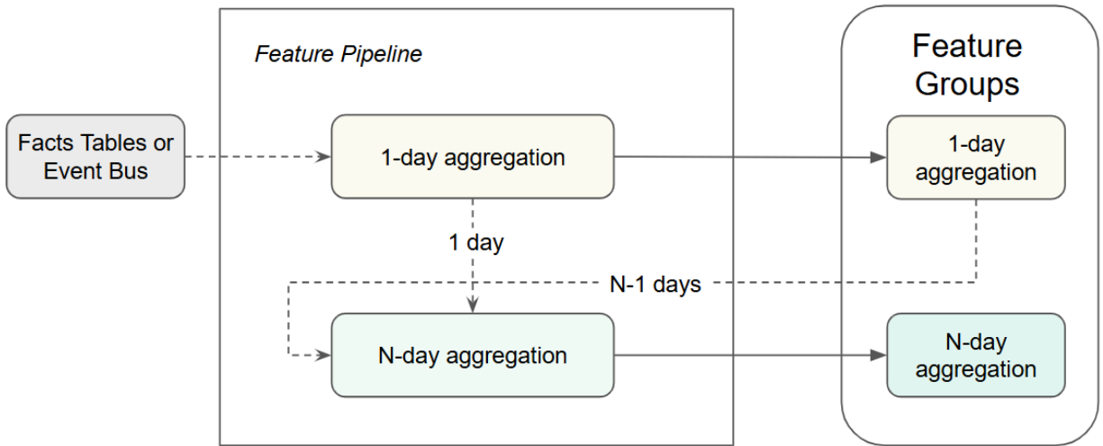
Figure 6-8. We can compute single-day and multi-day aggregations in the same feature pipeline. Multi-day aggregations combine the current daily aggregation with the historical daily aggregations read from the feature store.
