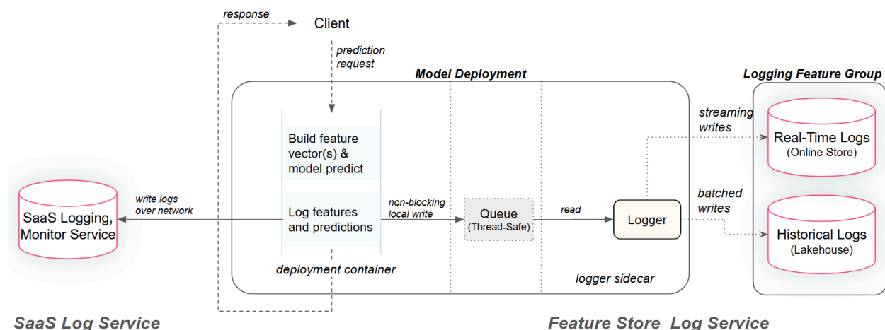
Figure 14-3. Architecture diagram comparing blocking and non-blocking logging services for a model deployment. The network hosted SaaS logging service has higher latency and can suffer from data loss if there are network or service availability problems. Non-blocking logging reduces prediction latency and increases robustness by having the logger in a separate thread of control.
