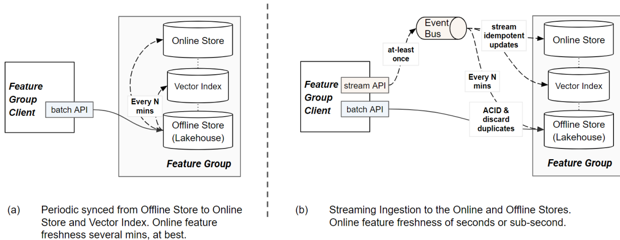
Figure 4-6. Two different feature store architectures. In (a) clients write to the offline feature store and updates are periodically synchronized to the online store and vector index. In (b) clients can also write via a stream API to an event streaming platform, after which updates are streamed to the online store and vector index, then periodically synchronized to the offline store.
