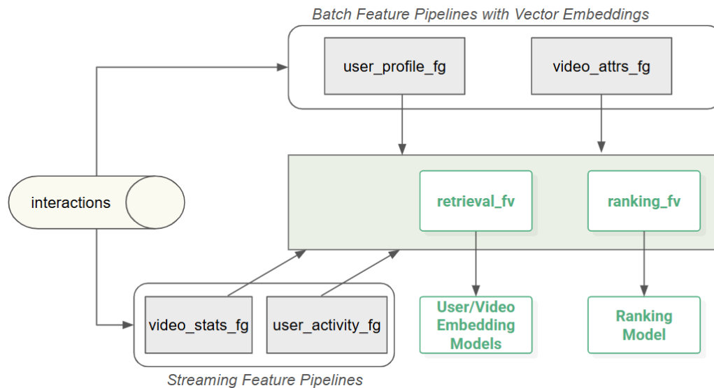
Figure 15-4. Feature Groups, Feature Views, and Models for our Video Recommender.
