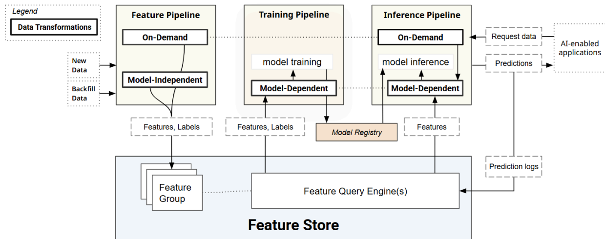
Figure 2-6. Data Transformations for Machine Learning and the ML Pipelines they are performed in
