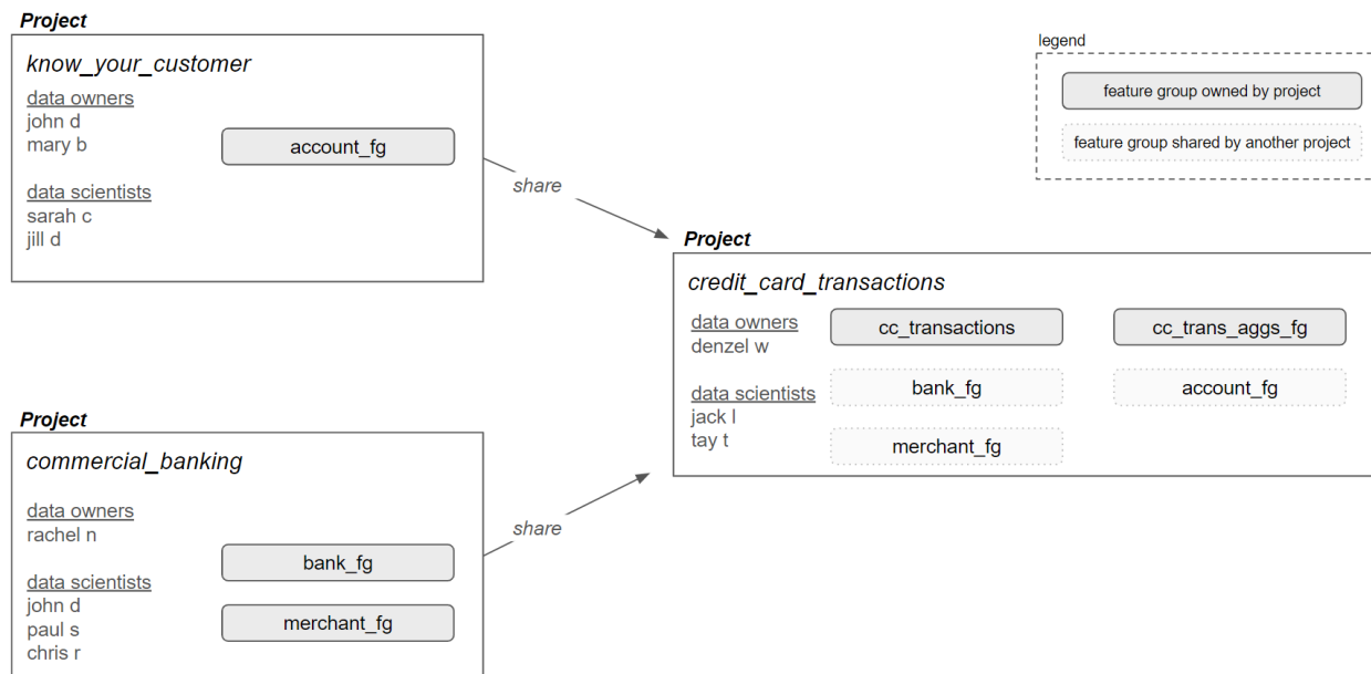
Figure 5-2. We refactored our project from Figure 5-1 to store our feature groups in 3 different projects. The new know_your_customer and commercial_banking projects share their feature groups (read-only) with the credit_card_transactions project. Members Jack, Tay, and Denzel of the credit_card_transactions project can now read feature data from all feature groups, but they can only write to the cc_trans_fg and cc_trans_aggs_fg feature groups.
