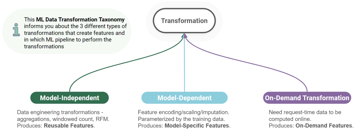
Figure 2-5. The taxonomy of Data Transformations for Machine Learning that create reusable features, model-specific features, and real-time features
