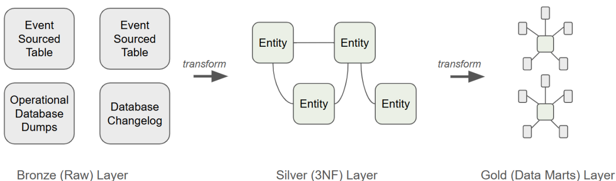
Figure 10-2. Data warehouses often have a medallion architecture, with bronze, silver, and gold layers. Features and labels for ML models may come from all layers, not just the gold layer.
